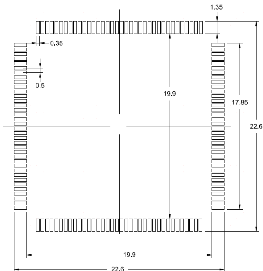
Figure 20 LQFP144 Layout Recommendations
