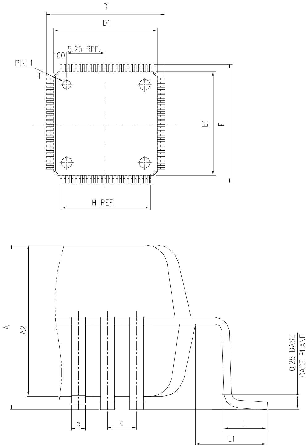
Figure 21 LQFP100 Package Diagram
