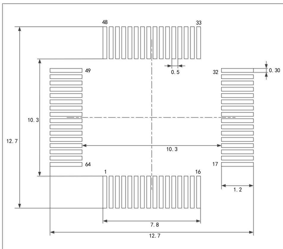
Figure 24 LQFP64 Welding Layout Recommendations
