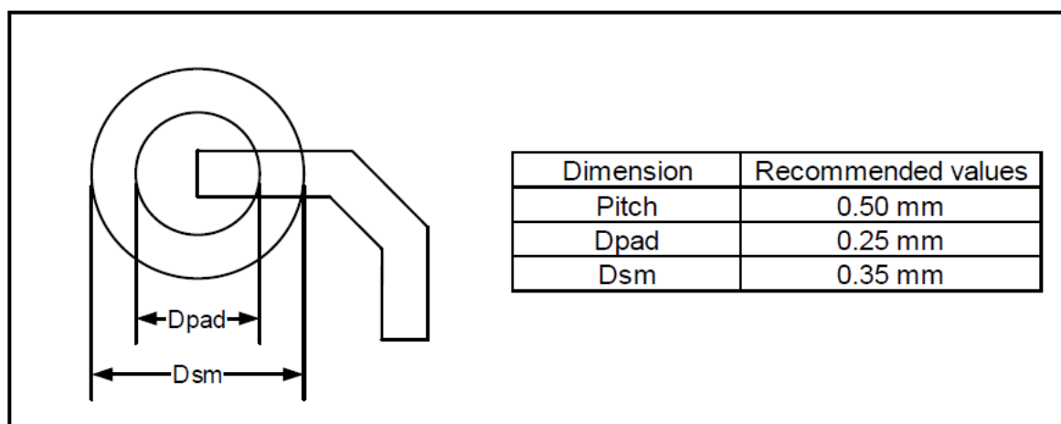
Figure 30 BGA100 Welding Layout Recommendations
