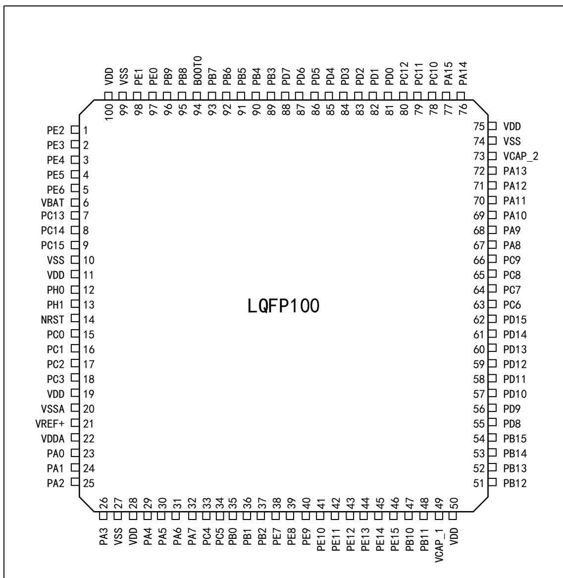
Figure 2 Distribution Diagram of APM32F427xG_F425xG_F423xG Series LQFP100 Pins
