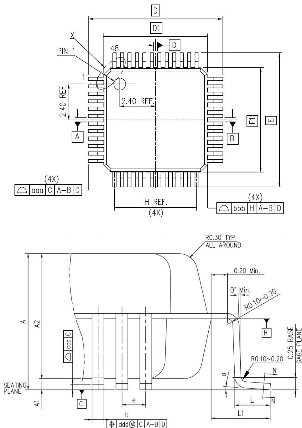
Figure 25 LQFP48 Package Diagram
