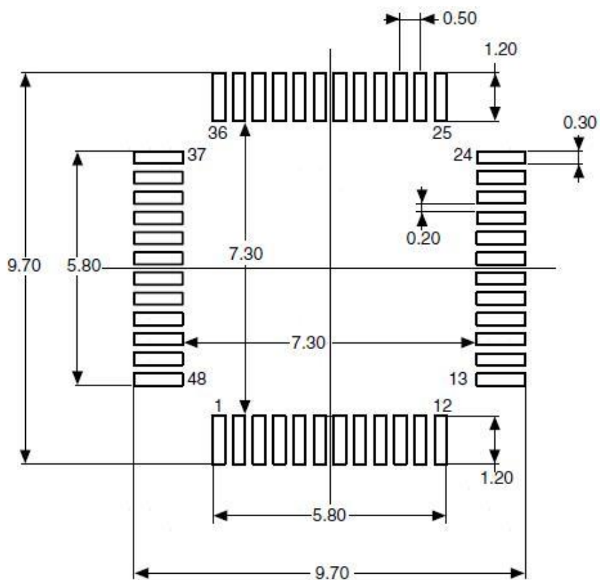
Figure 26 LQFP48 Welding Layout Recommendations
