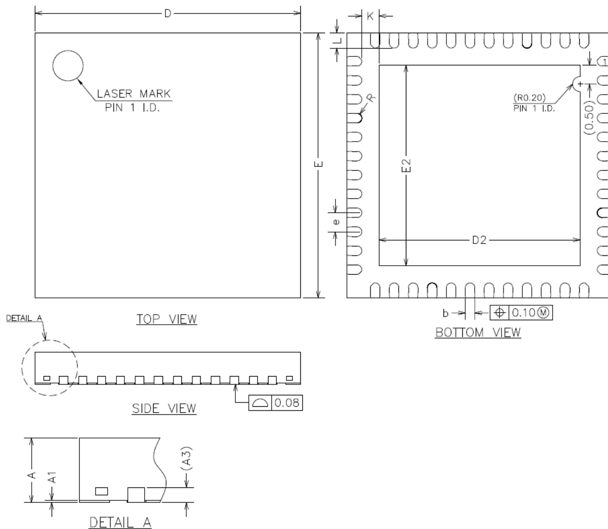
Figure 27 QFN48 Package Diagram
