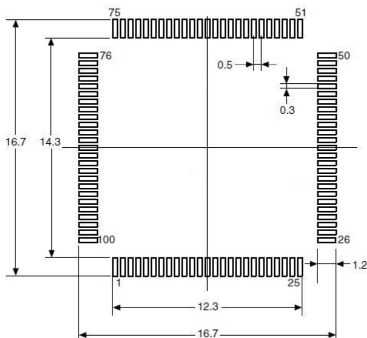
Figure 22 LQFP100 Welding Layout Recommendations
