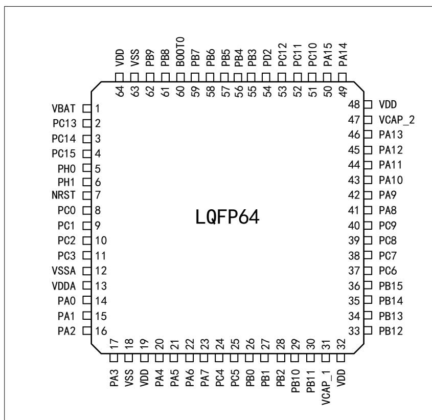
Figure 3 Distribution Diagram of APM32F427xG_F425xG_F423xG Series LQFP64 Pins
