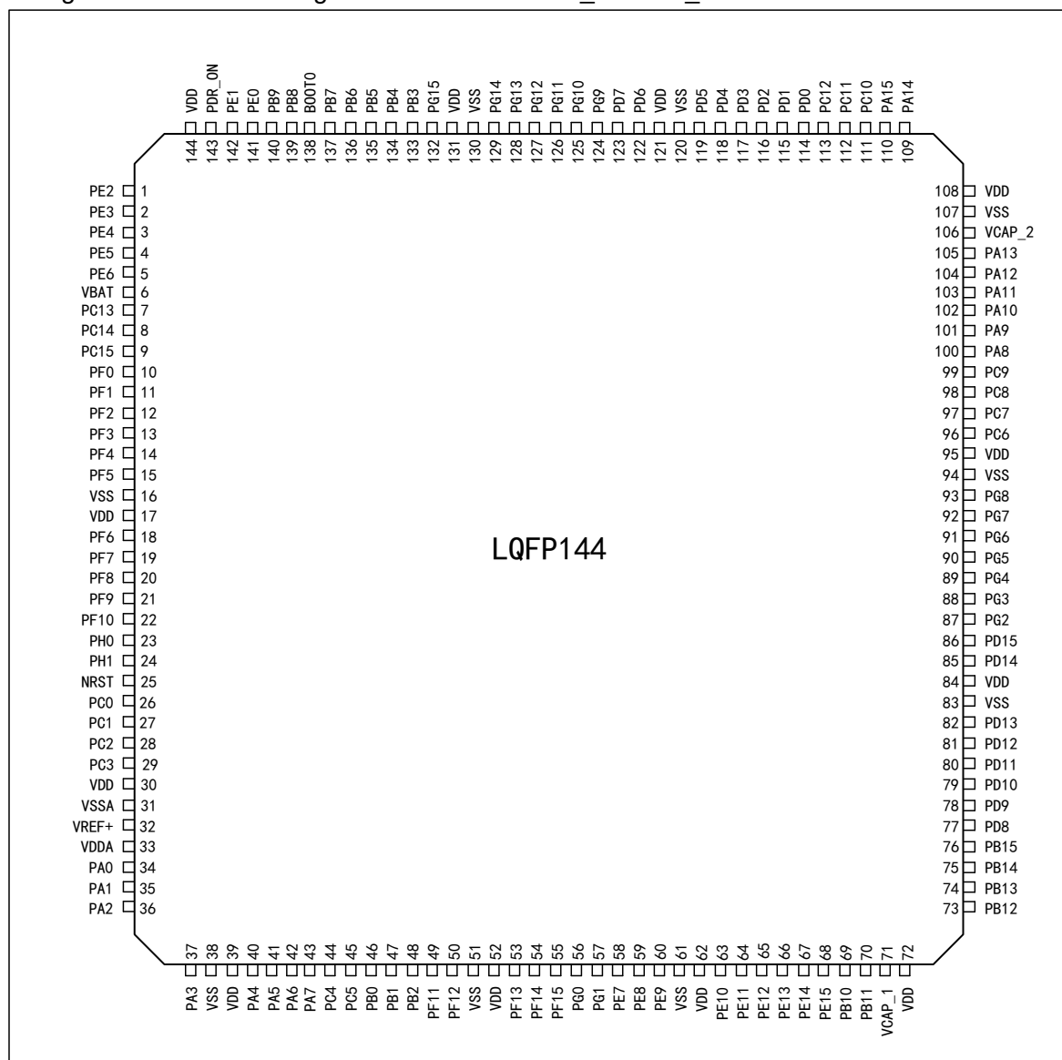
Figure 1 Distribution Diagram of APM32F427xG_F425xG_F423xG Series LQFP144 Pins
