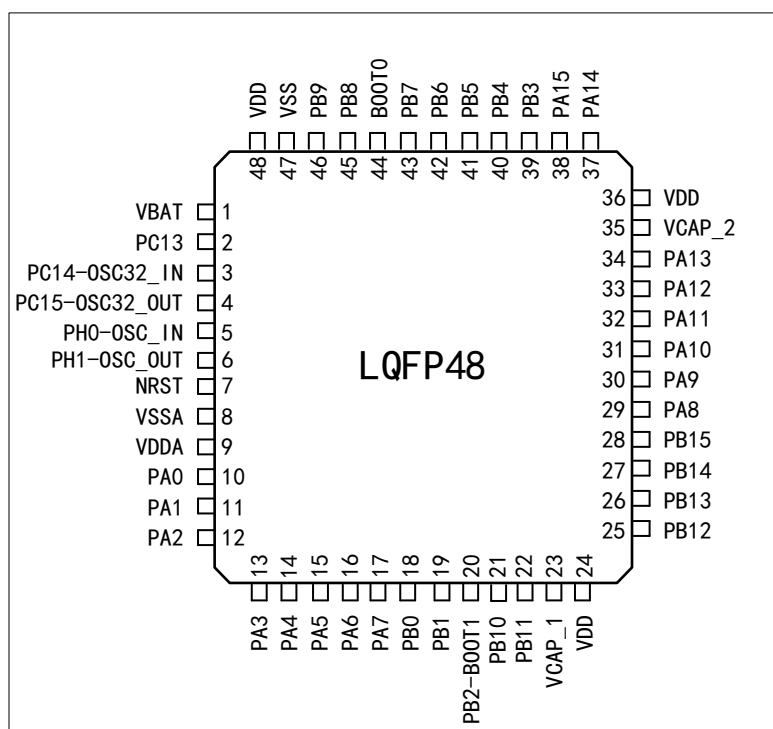
Figure 4 Distribution Diagram of APM32F427xG_F425xG_F423xG Series LQFP48 Pins
