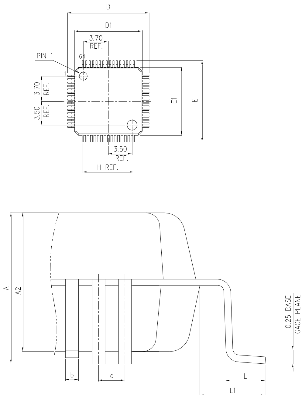
Figure 23 LQFP64 Package Diagram
