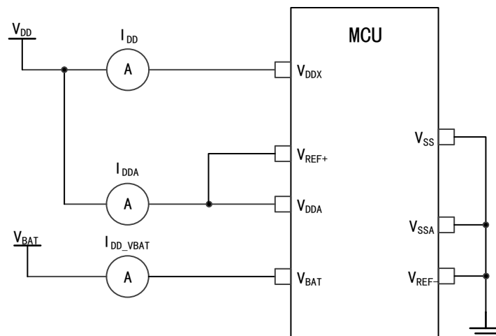
Figure 12 Power Consumption Measurement Scheme
