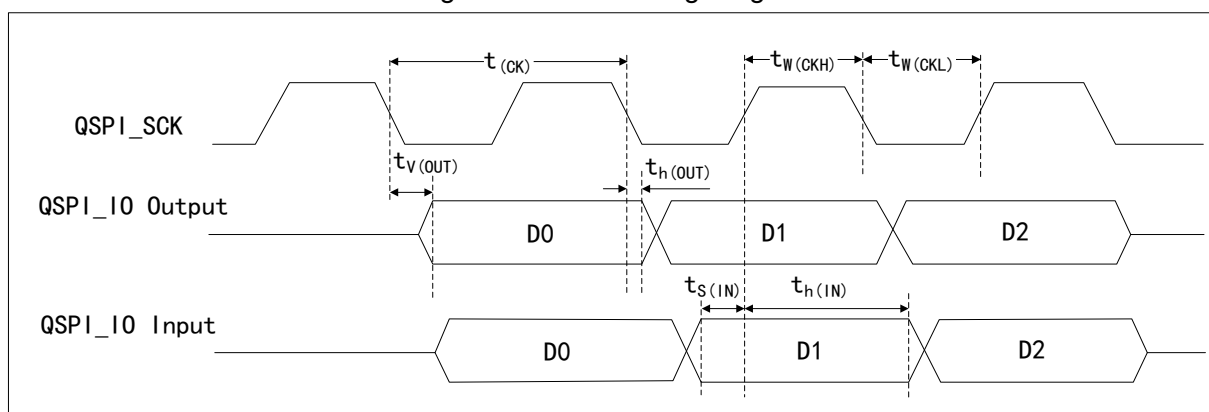
Figure 18 QSPI Timing Diagram
