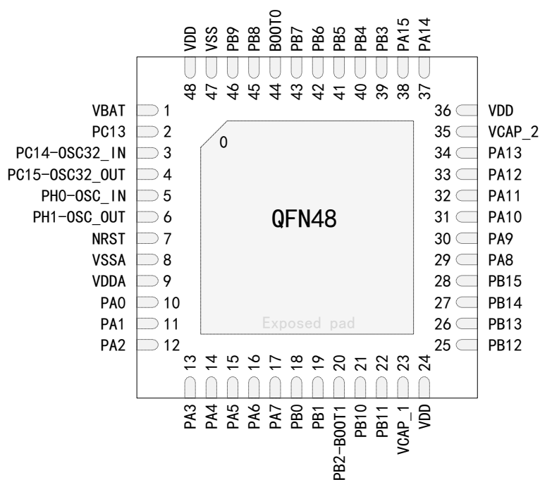
Figure 6 Distribution Diagram of APM32F427xG_F425xG_F423xG Series QFN48 Pins
