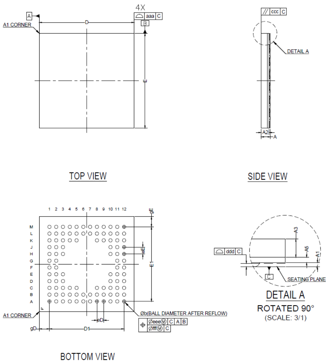
Figure 29 BGA100 Package Diagram
