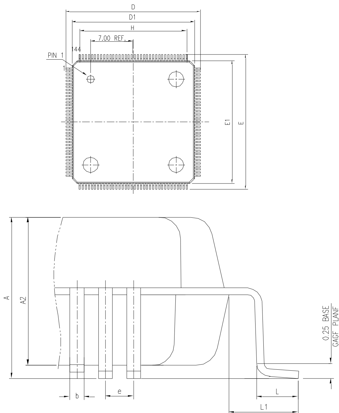
Figure 19 LQFP144 Package Diagram
