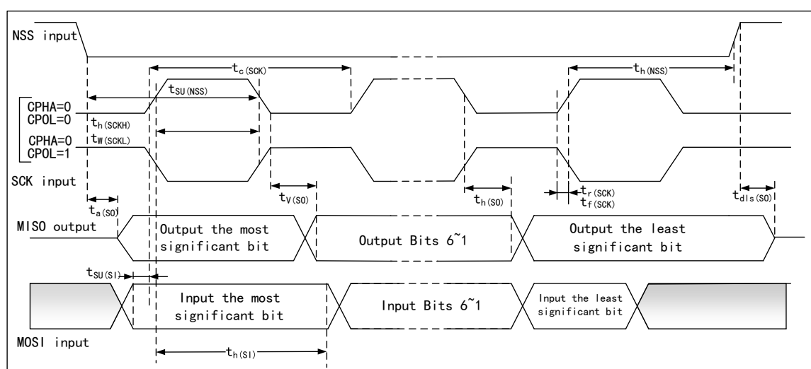
Figure 15 SPI Timing Diagram - Slave Mode and CPHA=0
