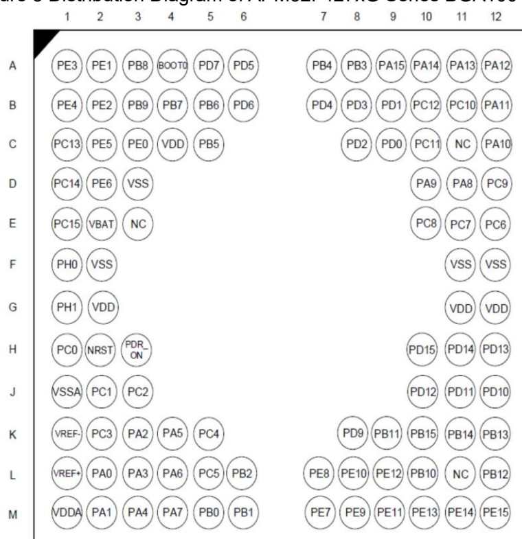
Figure 5 Distribution Diagram of APM32F427xG Series BGA100 Balls
