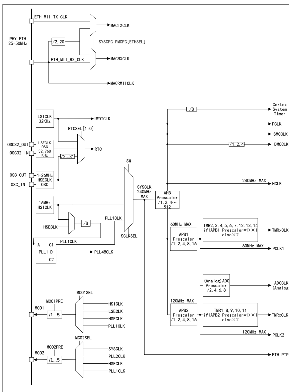
Figure 8 APM32F427xG_F425xG_F423xG Clock Tree
